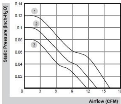
■ Air Flow-Static Pressure Characteristics
